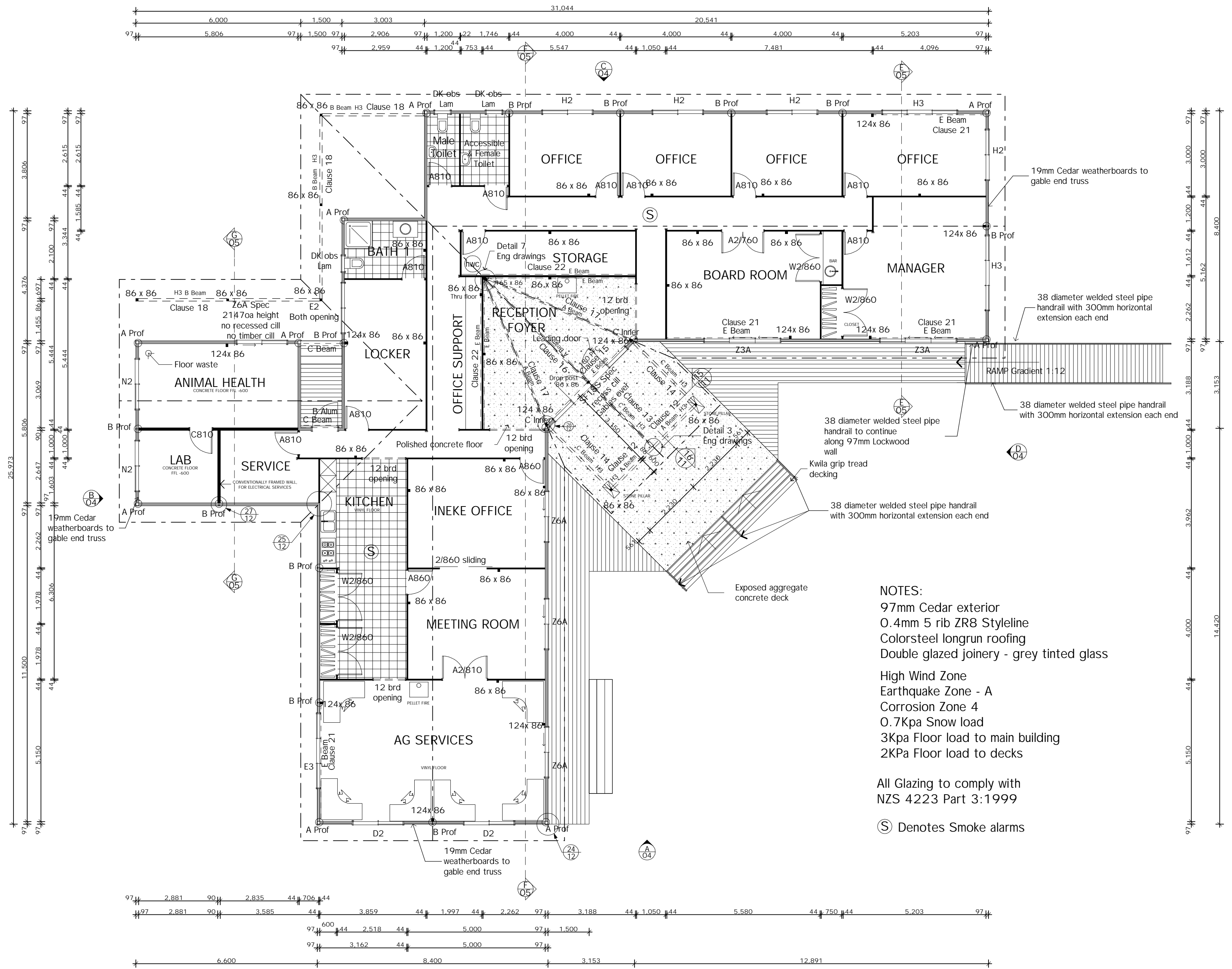
Floor Plan Scale 1:100 Area 373.52m 2
